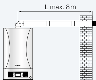
Horizontal connections
